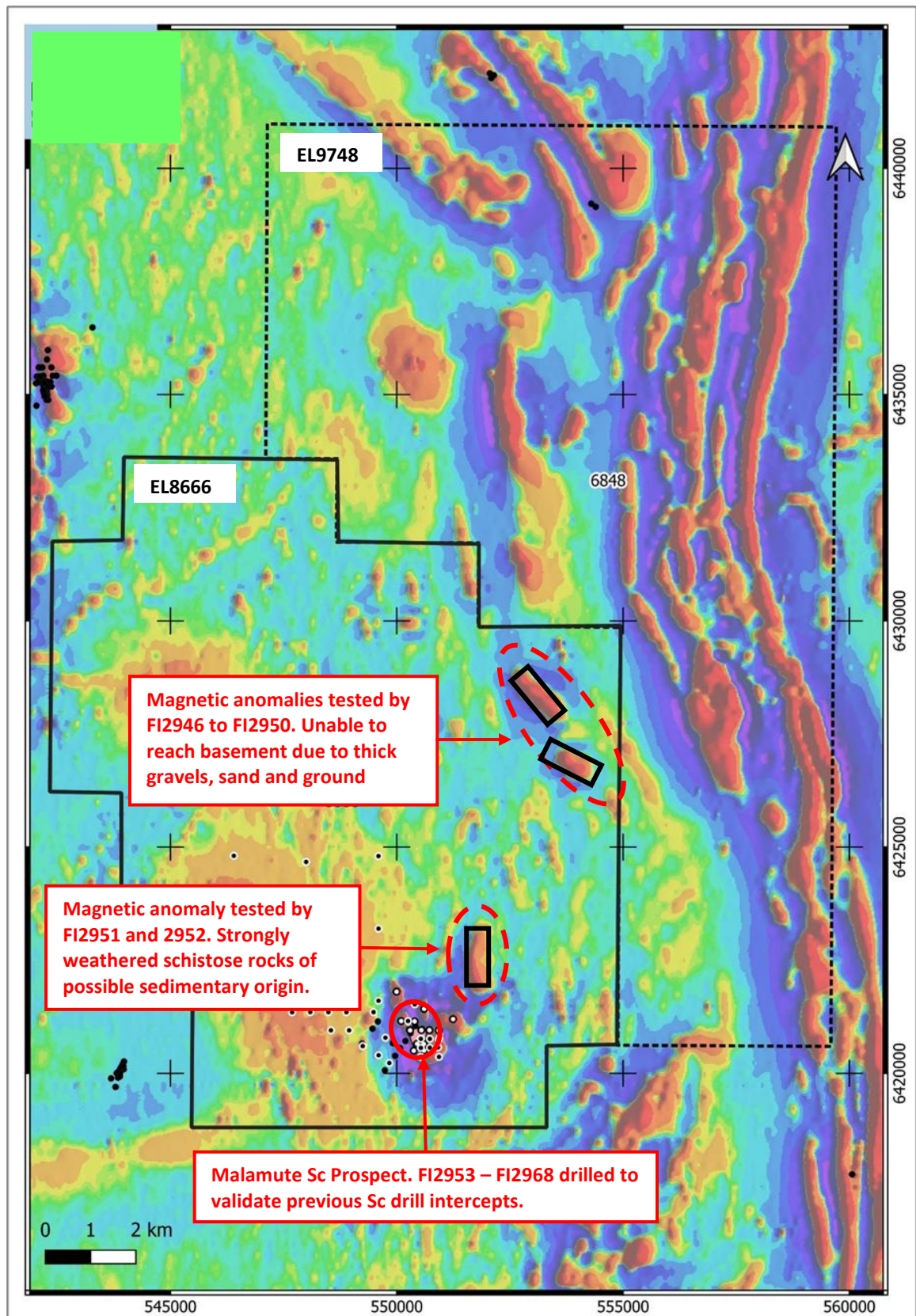
Figure 2: Rabbit Trap Scandium Project showing location of Malamute Scandium Prospect and magnetic anomalies drilled in December 2025. Historic drill holes shown as black dots.
