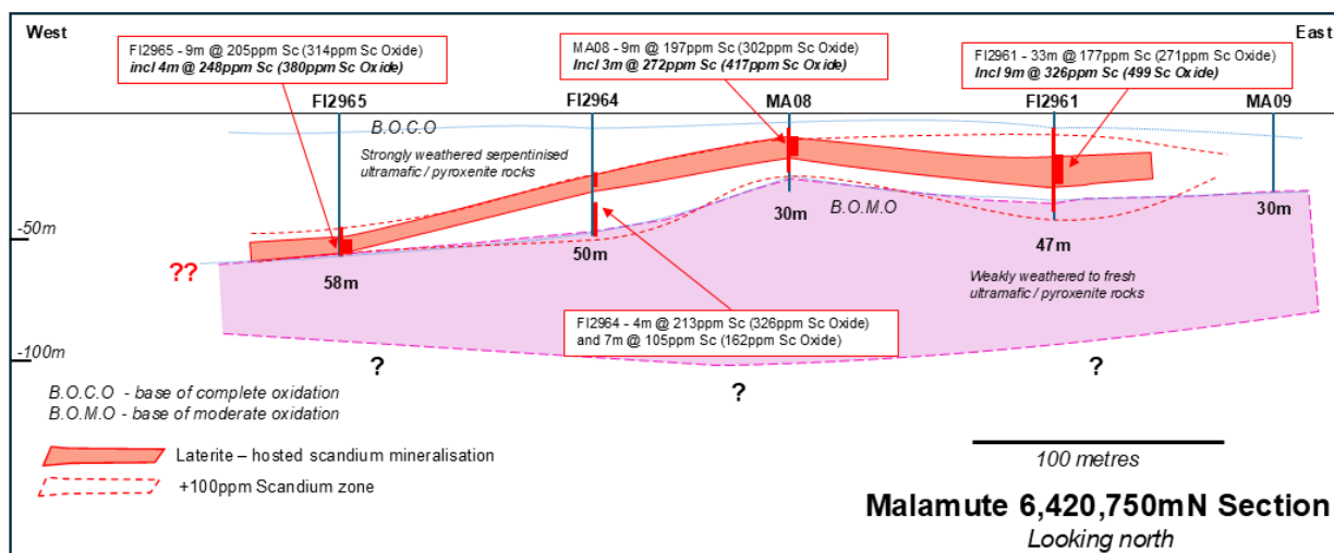
Figure 4: Malamute Scandium Prospect 6,420,750 cross section showing geology, weathering, and scandium mineralised zone. Section location shown on Figure 3 above.
