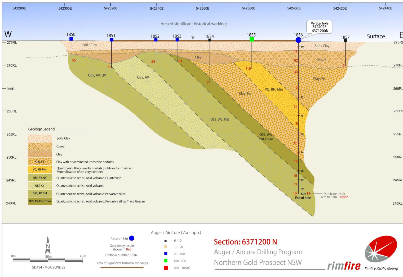
Figure 3: Northern Gold Interpreted Geological Section with Assays
