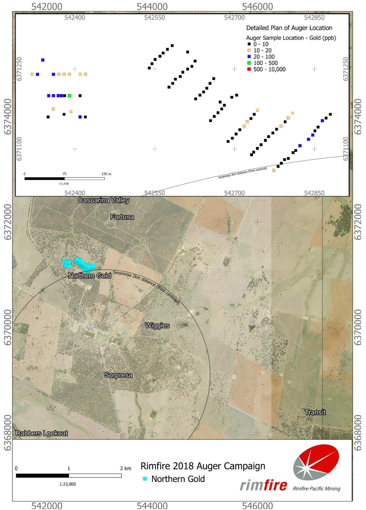
Figure 1: Northern Gold Location Plan
