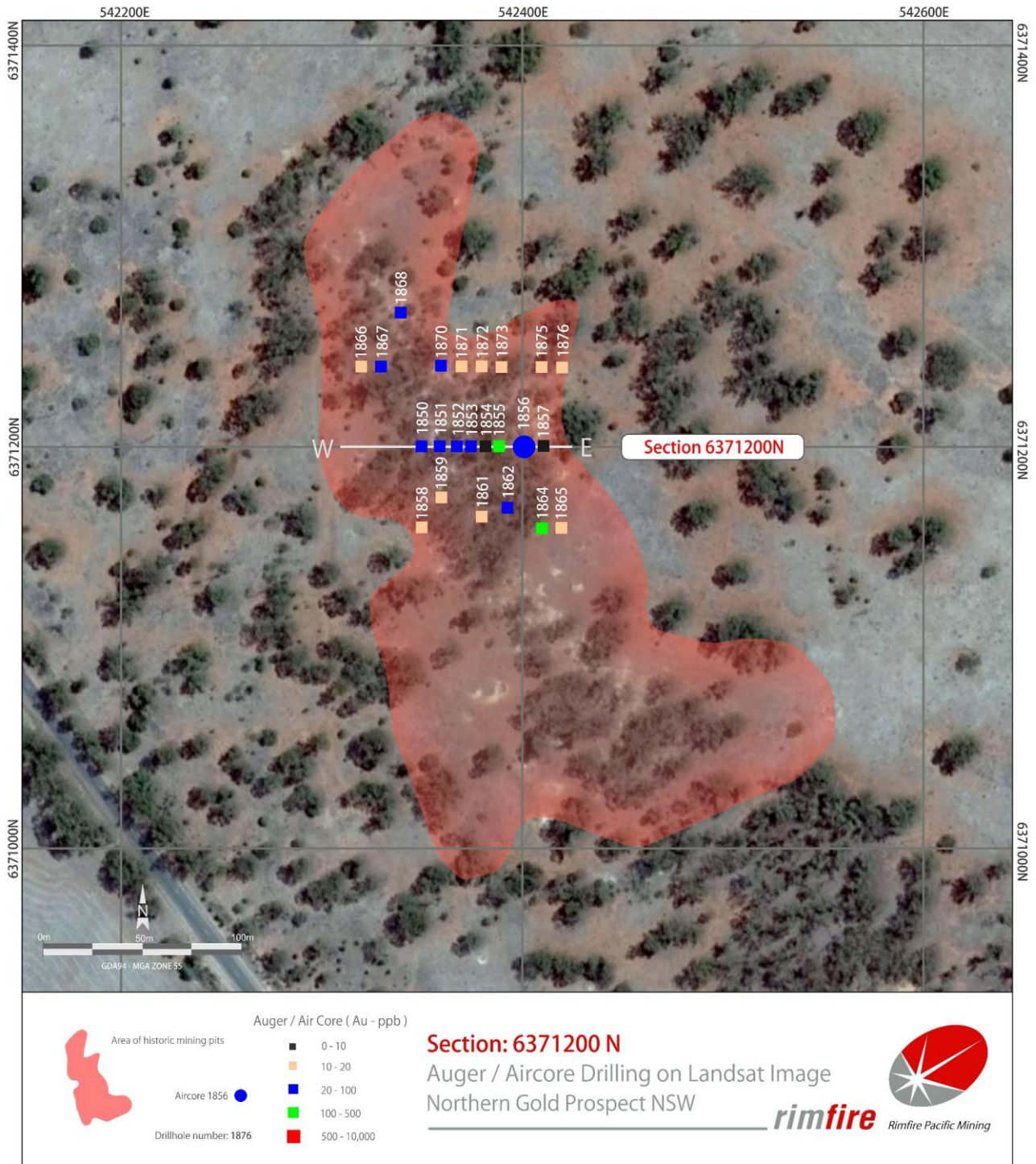
Figure 2: Northern Gold Sample Location Plan
