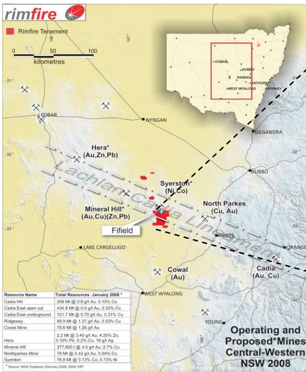
Regional Position for Fifield Mineralisation
