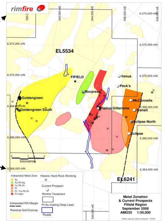
Fifield Mineralisation Metal Zoning Interpretation
